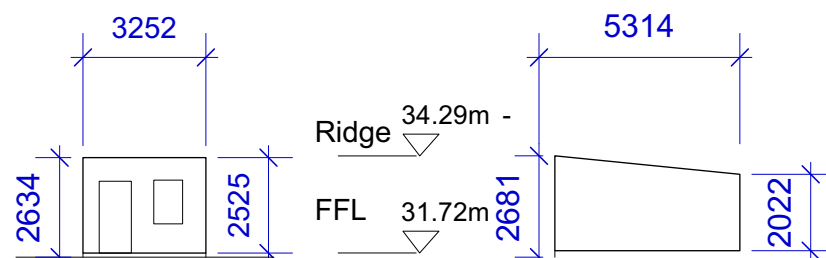
Elevation 2 North East
